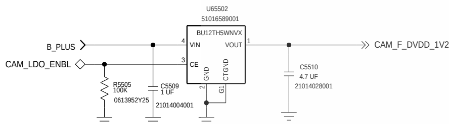
CAMERA CORE - 1.2V
